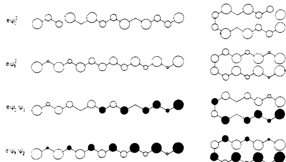
Figure 12. Charge density distributions e\psi_1^2 , e\psi_2^2 , e\psi_1\psi_1 , and e\psi_2\psi_2 in the hairpin and all-trans heptaenes. Circled areas are proportional to atomic charges (white: negative, black: positive).
