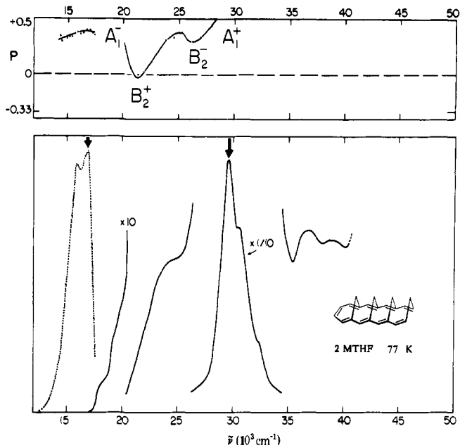
Figure 6. Spectra of the nonaene 6 in 2-methyltetrahydrofuran. See caption to Figure 1.
